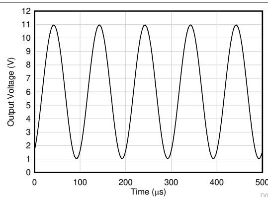
Figure 8-5. 2nd-Order MFB LP Filter DC Output
