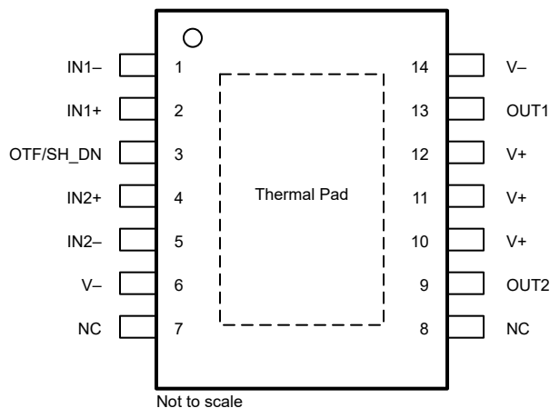
Figure 5-1. PWP Package, 14-Pin HTSSOP (Top View)
