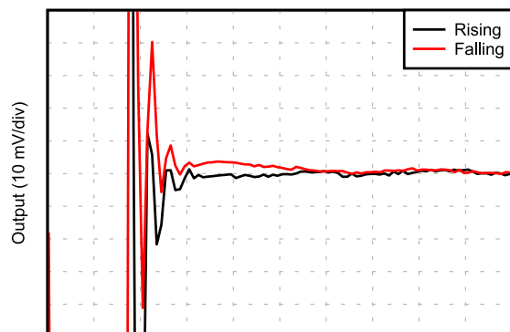
Figure 6-25. Settling Time
