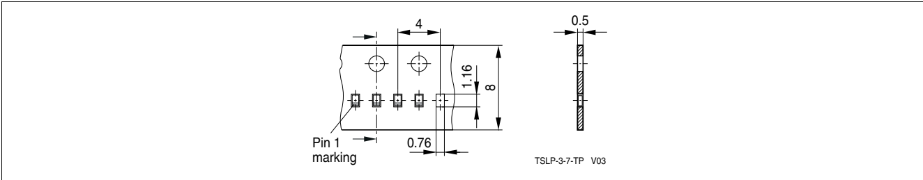
Figure 6-7 PG-TSLP-3-7: Packing
