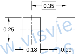
RECOMMENDED LAND PATTERN (Unit: mm)
