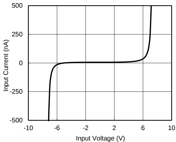
IV Curve
