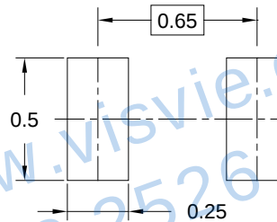
RECOMMENDED LAND PATTERN (Unit: mm)
