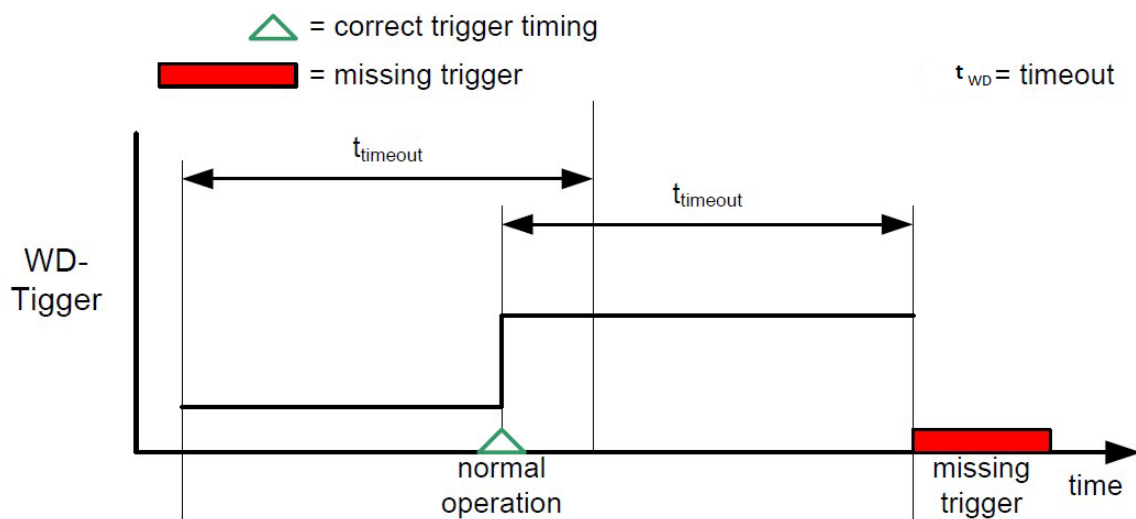
Figure 14. Timeout watchdog
