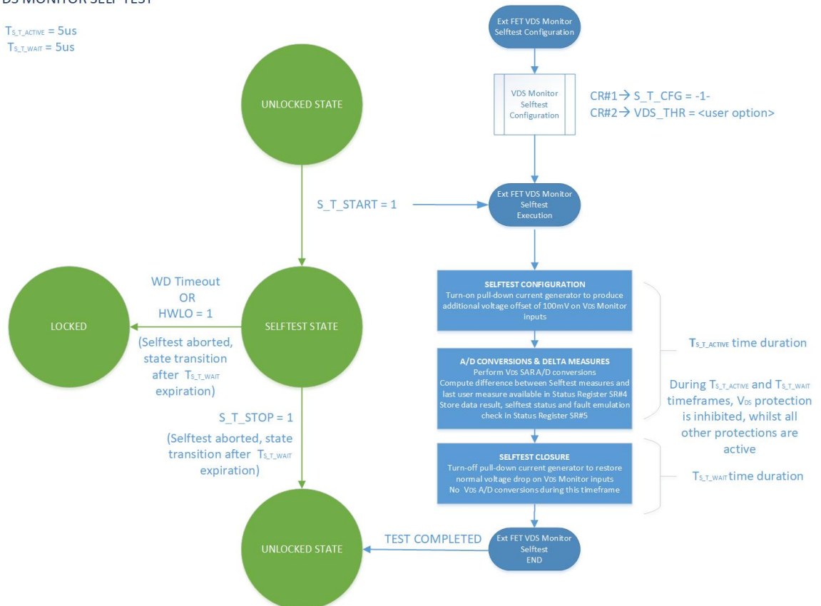
Figure 7. VDS monitor self test flow sequence
