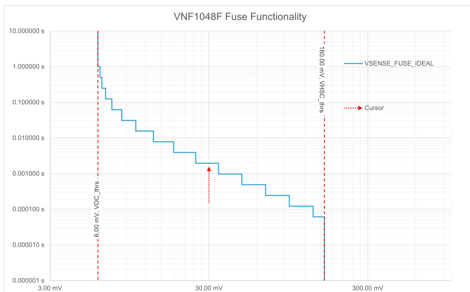
Figure 4. eFuse I 2 -t typical curve (VOC_thrs minimum - VHSC_thrs maximum)
