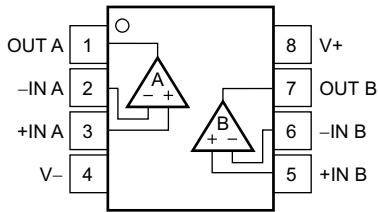
Pin Functions: OPA2348
