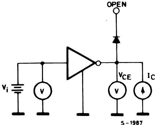
Figure 8. Input voltage
