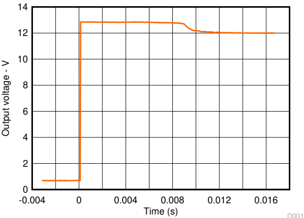
Figure 8-3. Output Response With De-activation of Coil (Turnoff)
