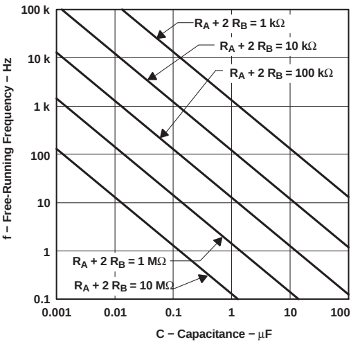
Figure 14. Free-Running Frequency
