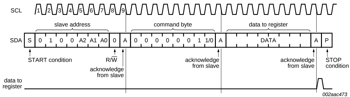
Fig 12. Write to Configuration register or Polarity Inversion register
