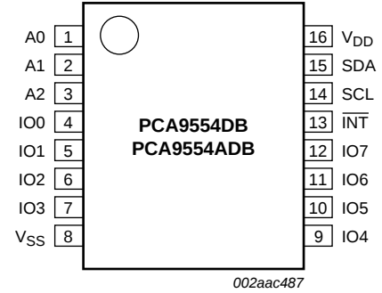
Fig 3. Pin configuration for SSOP16
