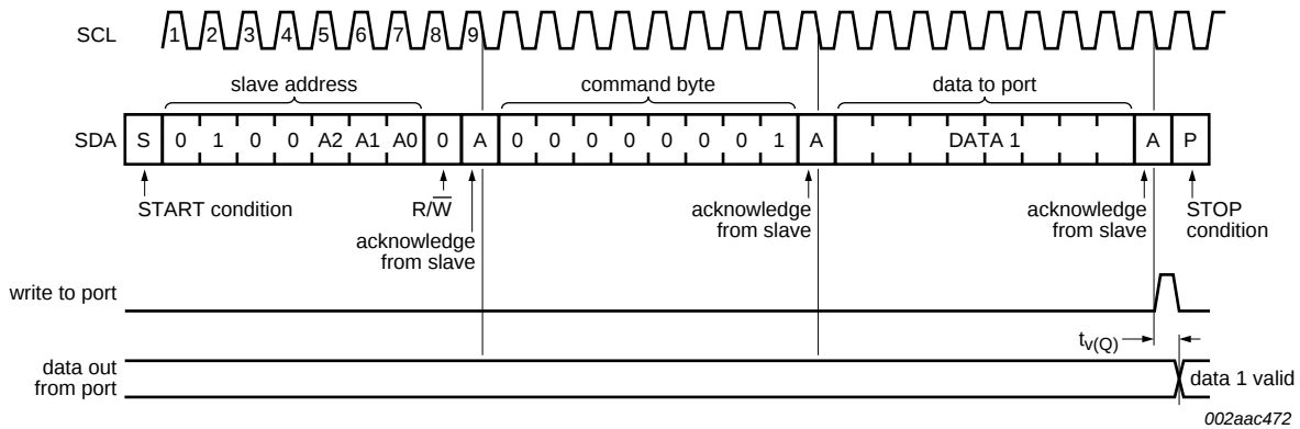
Fig 11. Write to Output Port register
