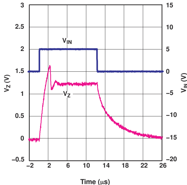
Figure 5-3. Start-Up Characteristics
