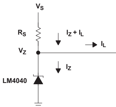
Figure 7. Shunt Regulator
