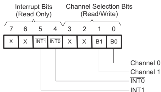
Figure 8-8. Control Register
