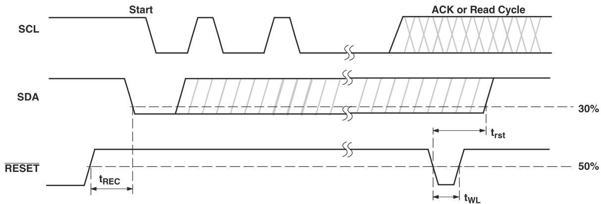
Figure 7-2. Reset Timing
