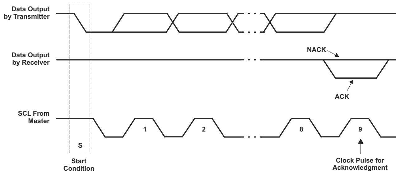
Figure 8-4. Acknowledgment on I²C Bus
