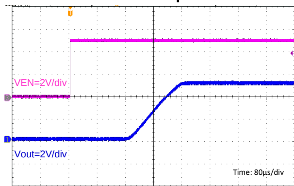
Enable Response
