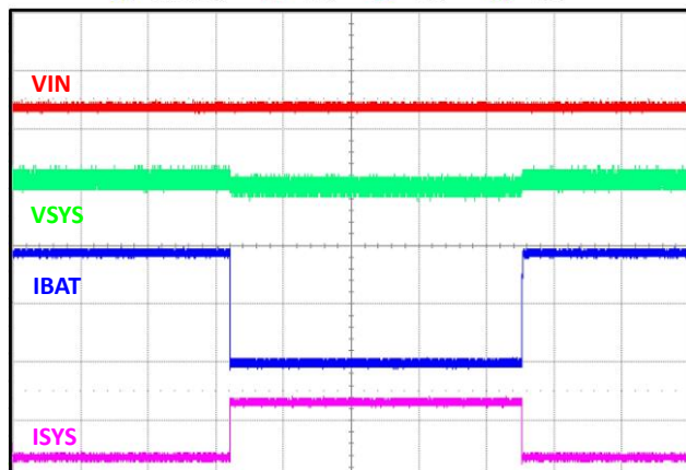
SYS Load Transient
