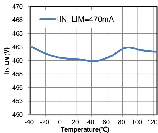
Figure 9 IIN_LIM vs. Temp,
