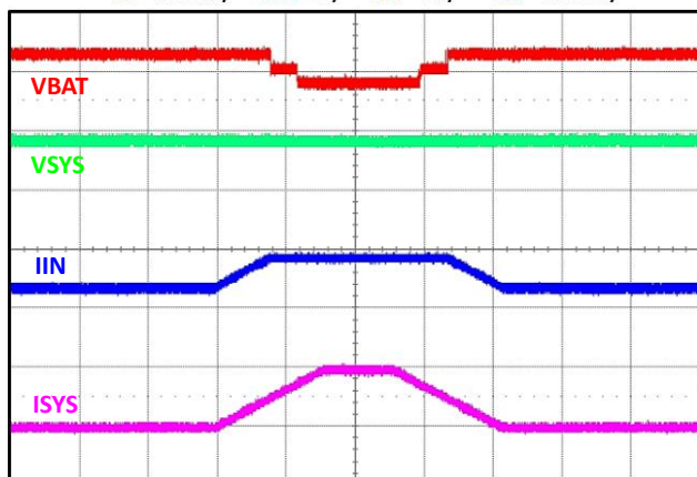
Input Current Limit-Based PPM
