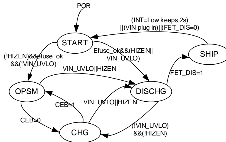
Figure 11 The main state machine conversion
