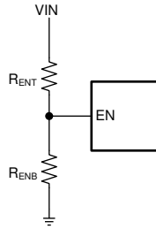
图 8-2. Setup for External UVLO Application
