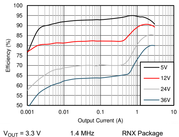
图 8-8. Efficiency
