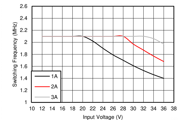
图 7-13. Switching Frequency versus Input Voltage V_{OUT} = 3.3\text{ V}
