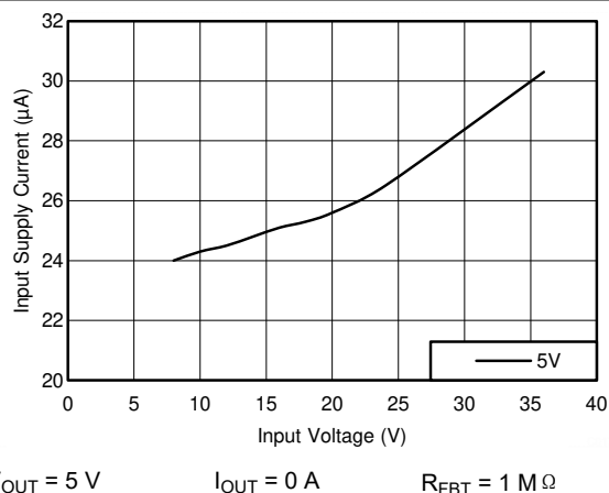
图 8-12. Input Supply Current
