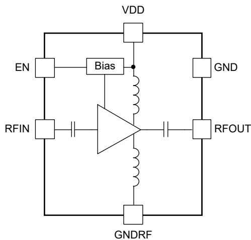
Figure 1. SGM13001A Block Diagram
