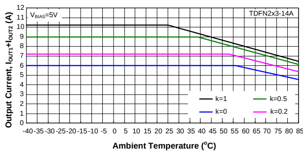
Figure 3. Derating Curves for APL3528 Package
