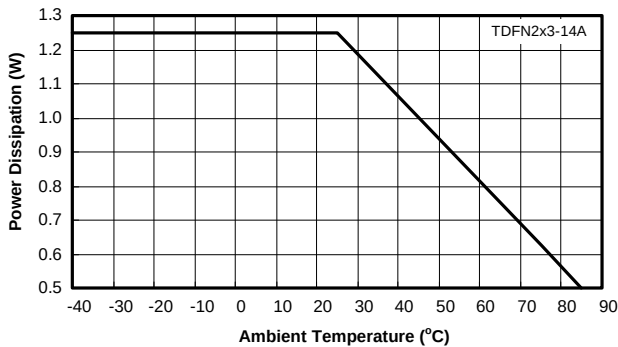
Figure 3. Derating Curves for APL3528 Package
