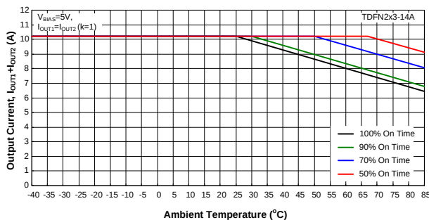
Figure 4. Safe Operating Area for APL3528 Package
