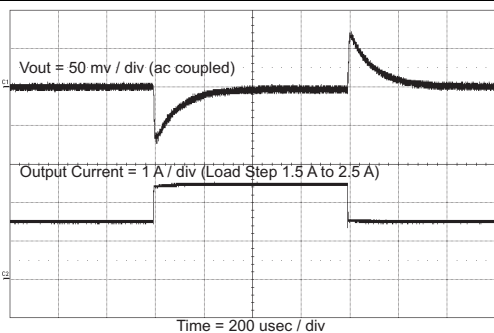
Figure 51. Load Transient
