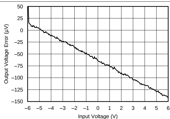
Figure 21. Measured Output Error with \pm 6 -V Input
