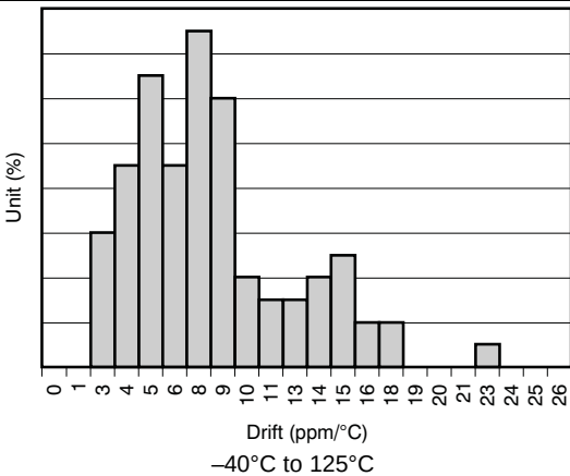
Figure 2. Temperature Drift
