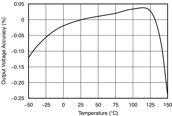
Figure 1. Temperature Drift
