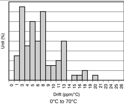
Figure 1. Temperature Drift
