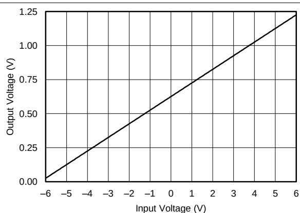
Figure 20. Measured DC Transfer Function with \pm 6 -V Input
