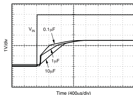
Figure 18. Start-Up Time
