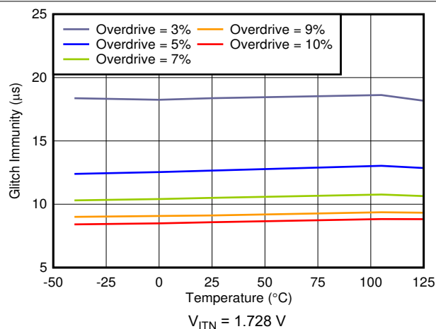
Figure 6-19. High-to-Low Glitch Immunity vs Temperature
