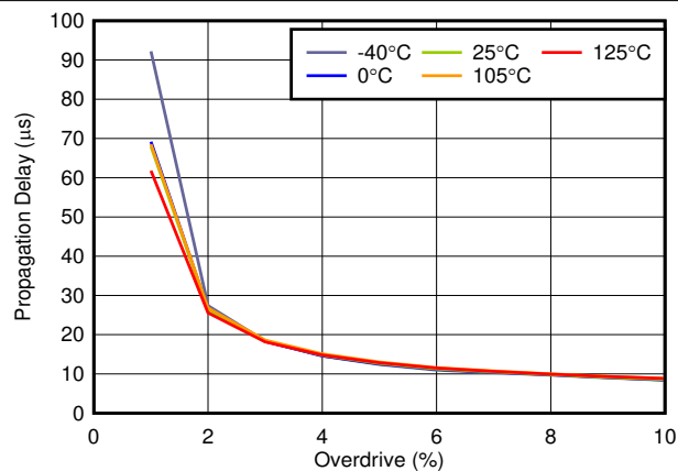
TPS3851G18 entering undervoltage Figure 6-15. Propagation Delay vs Overdrive
