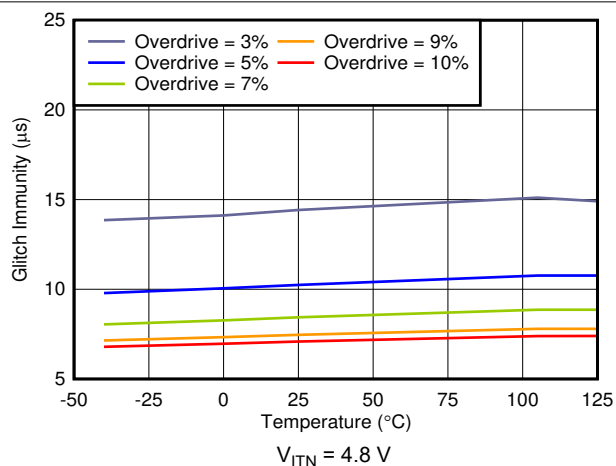
Figure 6-20. High-to-Low Glitch Immunity vs Temperature
