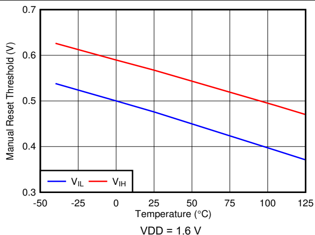
Figure 6-4. \overline{MR} Threshold vs Temperature
