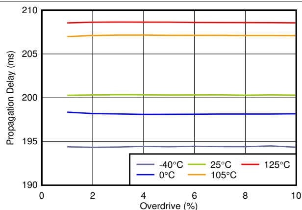
TPS3851G18 exiting undervoltage Figure 6-17. Propagation Delay ( t_{RST} ) vs Overdrive
