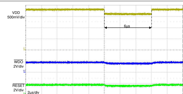
Figure 8-8. High-to-Low Glitch Immunity
