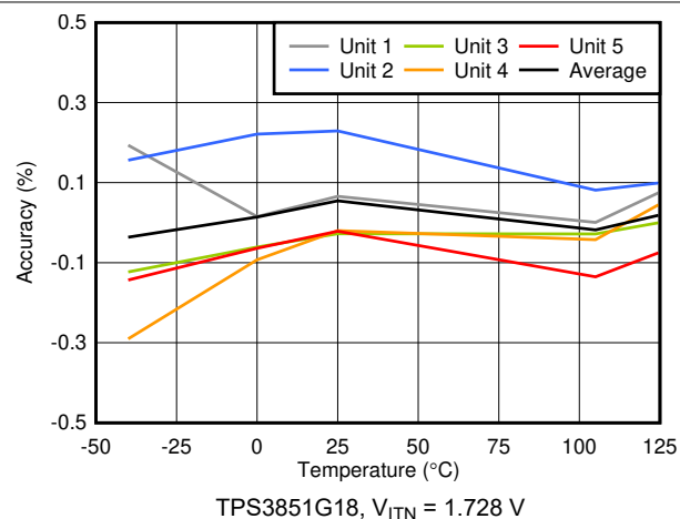
Figure 6-6. V_{ITN} + V_{HYS} Accuracy vs Temperature
