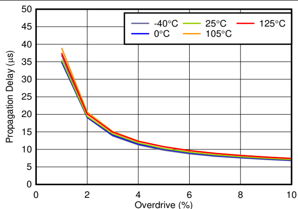
TPS3851G50 entering undervoltage Figure 6-16. Propagation Delay vs Overdrive
