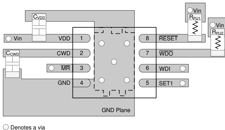
Figure 10-1. TPS3851 Recommended Layout
