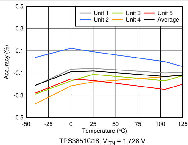
Figure 6-7. V_{ITN} Accuracy vs Temperature
