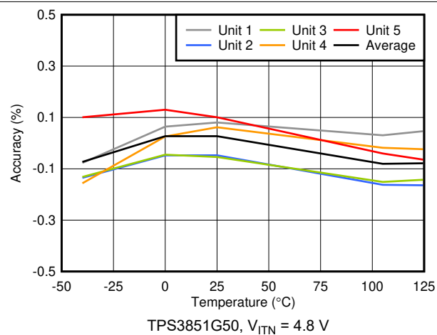
Figure 6-8. V_{ITN} + V_{HYS} Accuracy vs Temperature
