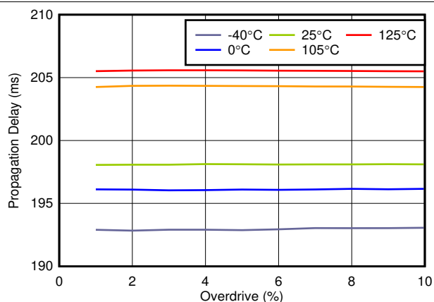
TPS3851G50 exiting undervoltage Figure 6-18. Propagation Delay ( t_{RST} ) vs Overdrive
