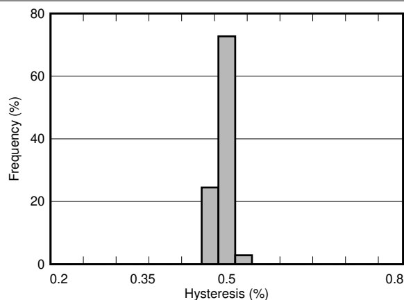
Figure 6-10. V_{ITN} + V_{HYST} Accuracy Histogram
