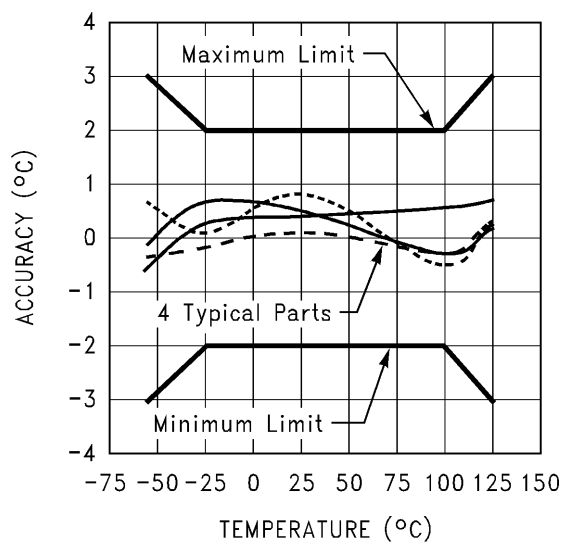
Figure 10. Temperature Accuracy
