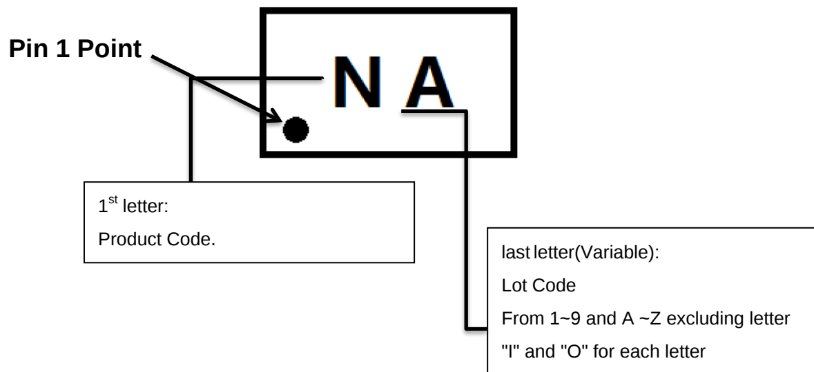
Figure 3. Marking specification (Top View)
