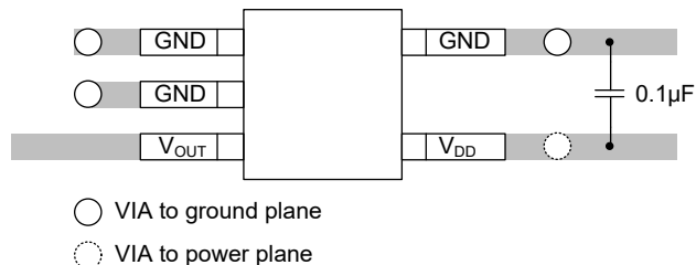
Figure 4. Recommended Layout: SC70-5 Package
