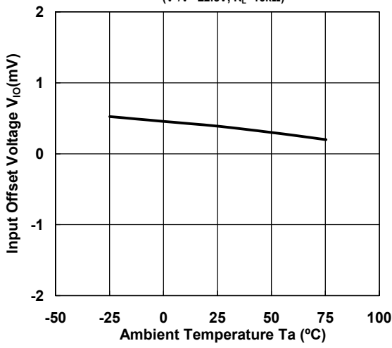
Input Offset Voltage vs. Temperature ( V^+/V^- = \pm 2.5V , R_L = 10k\Omega )
