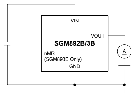
Test Circuit 3
