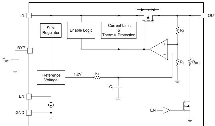
Figure 5. Internal Block Diagram of Low Noise Fixed Regulator (SOIC-8 Version)
