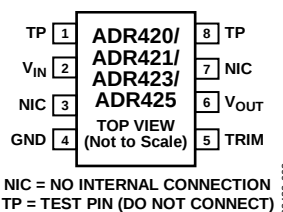
Figure 2. 8-Lead SOIC, 8-Lead MSOP Pin Configuration
