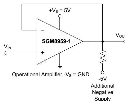
Figure 2. For V_{OUT} Range to Ground
