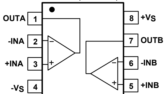
SGM722 (TOP VIEW)
