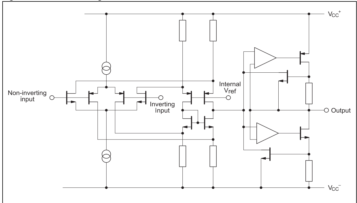
Figure 1. Schematic diagram
