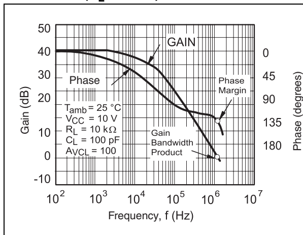
Figure 8. Gain and phase vs. frequency ( R_L = 10\text{ k}\Omega )
