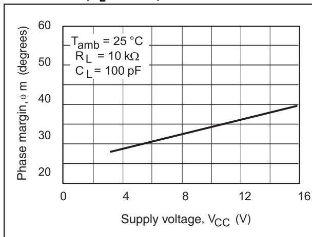
Figure 10. Phase margin vs. supply voltage ( R_L = 10\text{ k}\Omega )
