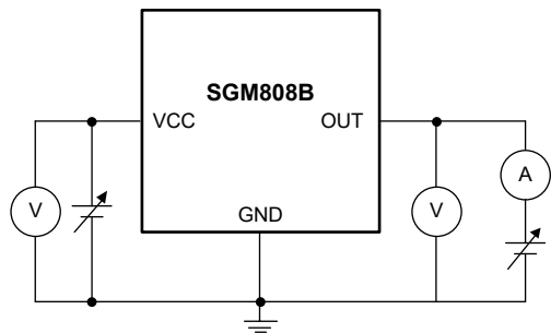
Test Circuit 3
