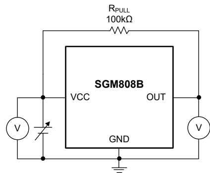
Test Circuit 1
