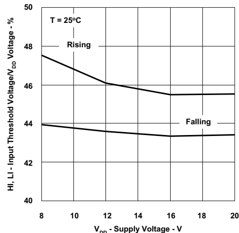
Figure 6. UCC27200 Input Threshold vs Supply Voltage
