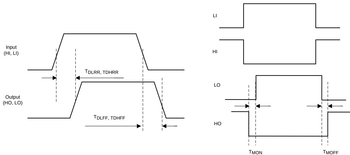
Figure 1. Timing Diagrams
