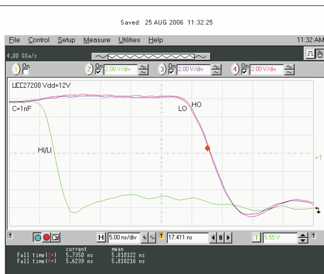
Figure 27. V_{LO} and V_{HO} Fall Time, 1-nF Load, 5 ns/Div
