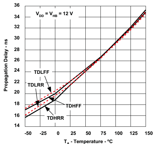
Figure 15. UCC27201 Propagation Delays vs Temperature
