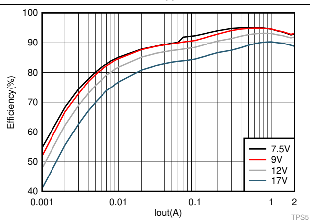
图 8. TPS562231 V_{OUT} = 1.8\text{ V} Efficiency
