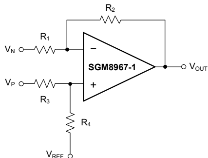
Figure 5. Difference Amplifier
