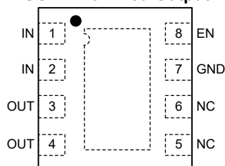
TDFN-3x3-8L
