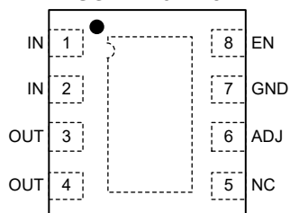
TDFN-3x3-8L
