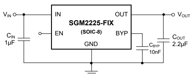
Figure 2. Low Noise Regulator (Fixed Voltage Version)
