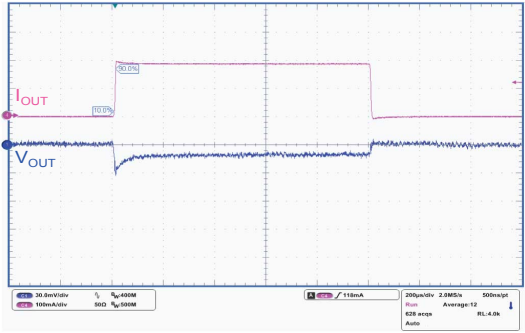
Figure 28. Load transient ( V_{OUT} = 5\text{ V} )
