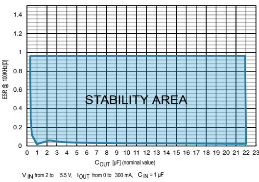
Figure 18. Stability area vs. ( C_{OUT} , ESR)
