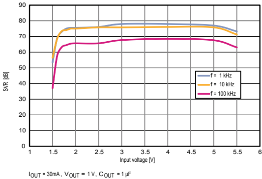
Figure 16. Supply voltage rejection vs. input voltage
