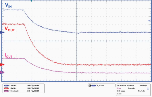
Figure 24. Turn-off time ( V_{OUT} = 5\text{ V} )
