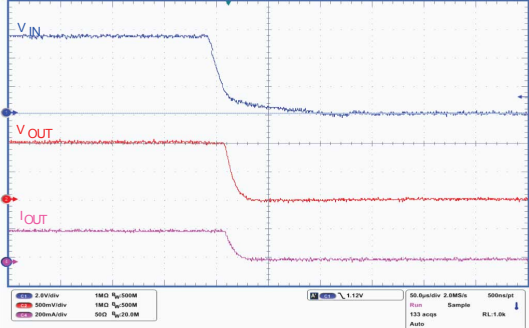
Figure 22. Turn-off time ( V_{OUT} = 1\text{ V} )
