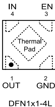
Figure 3. Pin connection (top view)
