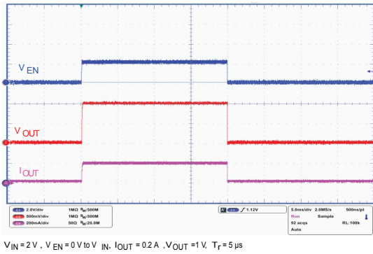
Figure 19. Enable startup ( V_{OUT} = 1\text{ V} )
