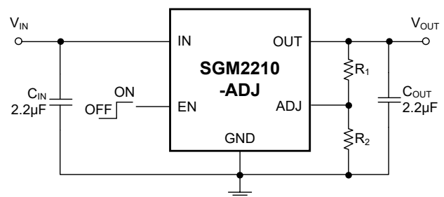
Adjustable Output Voltage Version
