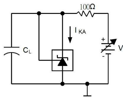
Test Circuit For Curve A
