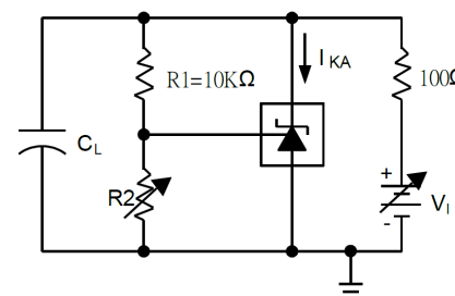
Test Circuit For Curve B
