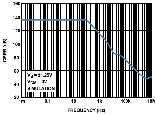
FIGURE 35. CMRR vs FREQUENCY, V_S = 2.5\text{V}
