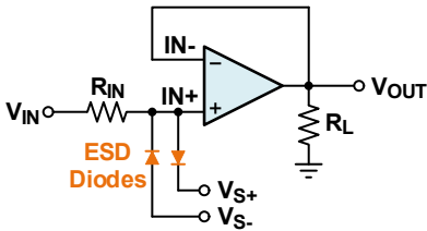
FIGURE 45. INPUT CURRENT LIMITING
