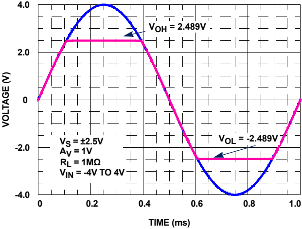
FIGURE 63. SIMULATED NO PHASE INVERSION, VOH AND VOL
