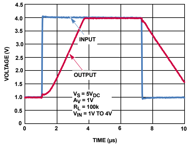
FIGURE 58. CHARACTERIZED LARGE SIGNAL STEP RESPONSE (3V)
