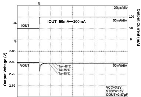
Fig 199. Load Response
