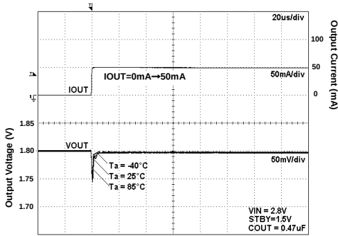
Fig 64. Load Response
