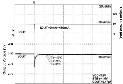
Fig 193. Load Response
