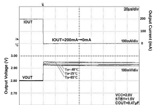
Fig 198. Load Response
