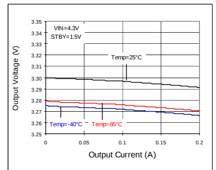
Fig 264. Load Regulation
