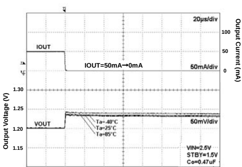
Fig 15. Load Response
