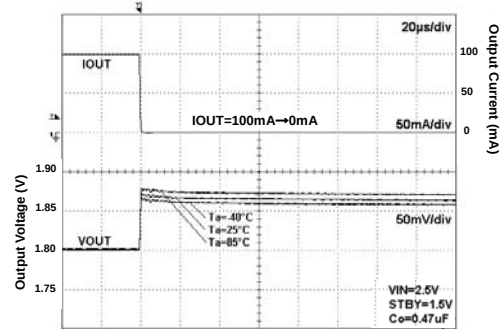
Fig 67. Load Response
