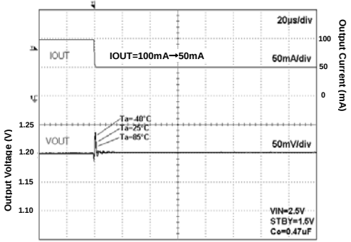
Fig 21. Load Response
