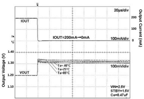
Fig 19. Load Response
