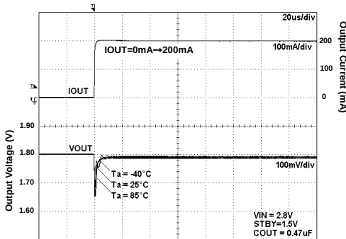
Fig 68. Load Response
