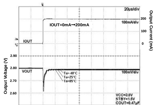
Fig 197. Load Response
