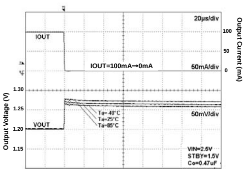
Fig 17. Load Response
