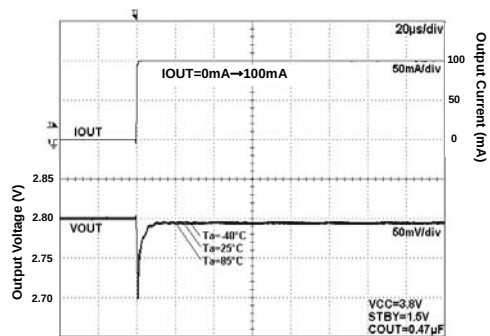
Fig 195. Load Response
