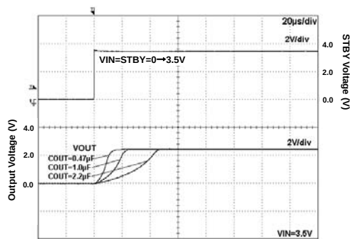
Fig 125. Start Up Time (VIN=STBY) Iout=0mA Iout=0mA
