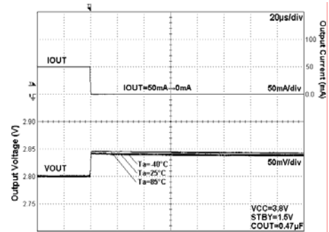
Fig 194. Load Response
