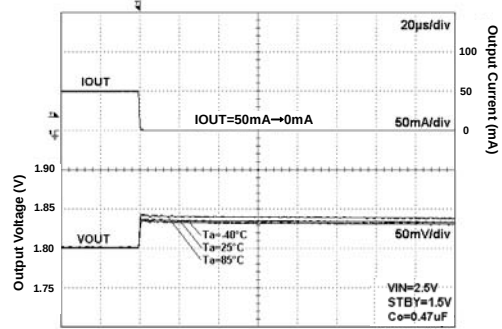
Fig 65. Load Response
