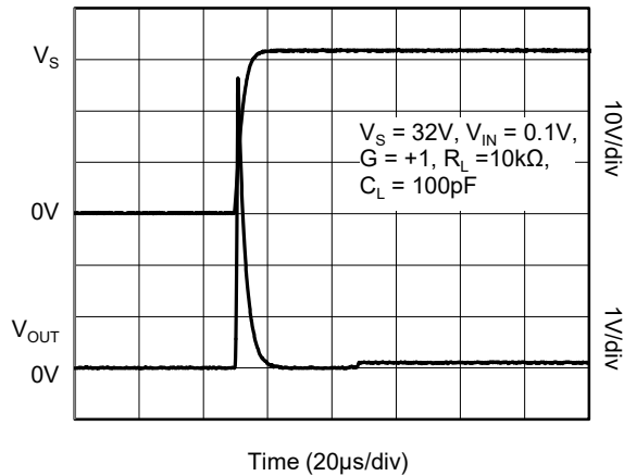
Turn-On Time
