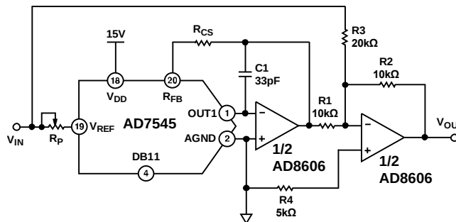
Figure 59. Bipolar Operation
