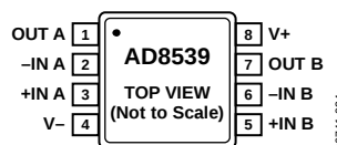
Figure 4. 8-Lead MSOP (RM-8)
