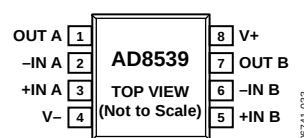
Figure 3. 8-Lead SOIC_N (R-8)
