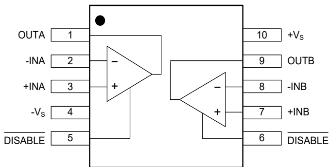
MSOP-10
