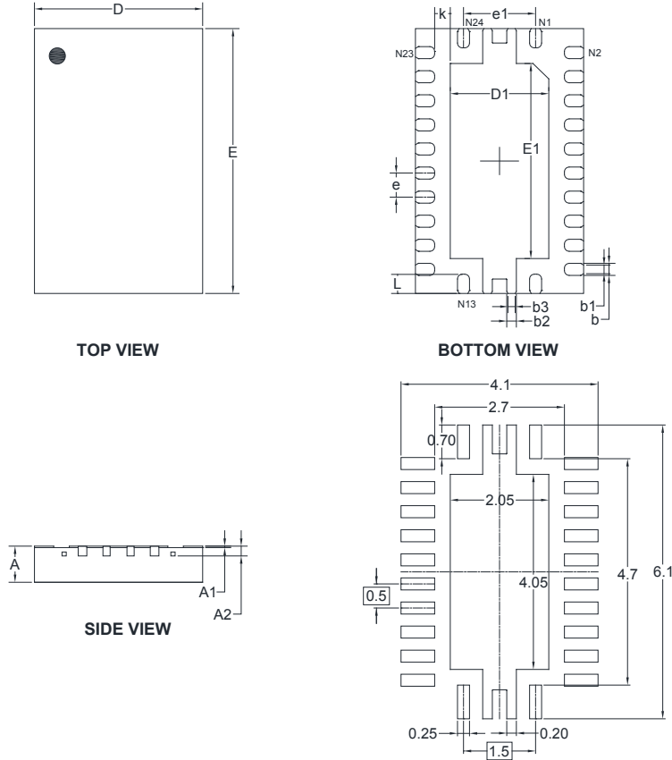
RECOMMENDED LAND PATTERN (Unit: mm)
