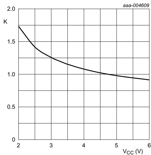
Fig 15. Typical K-factor for relaxation oscillator
