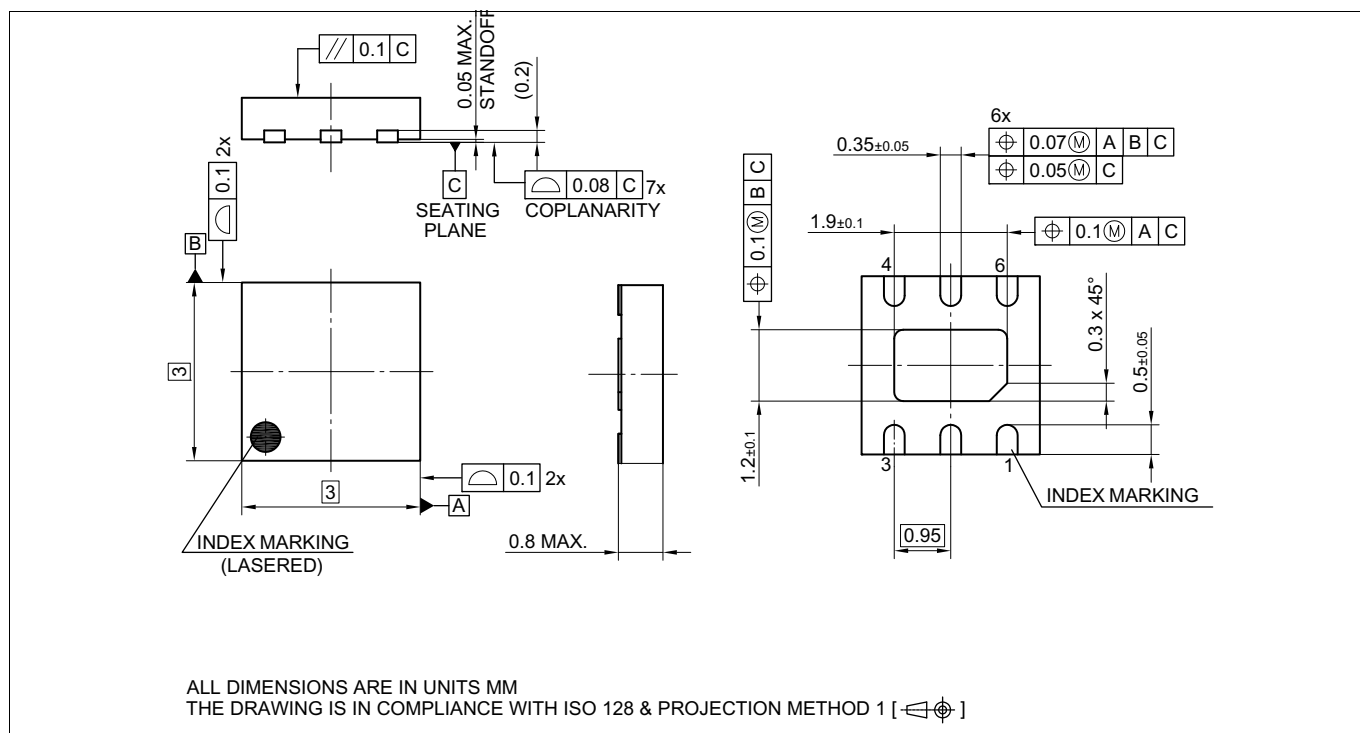
Figure 23 PG-WSN-6-1 Outline Dimensions
