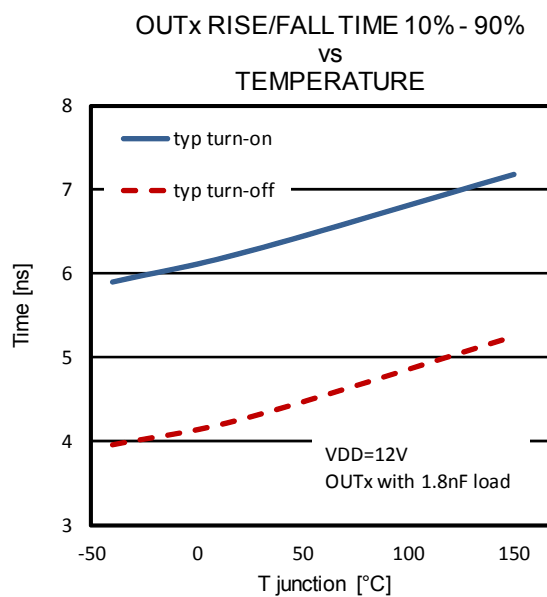
Figure 14 Rise / Fall Times with Load on Output
