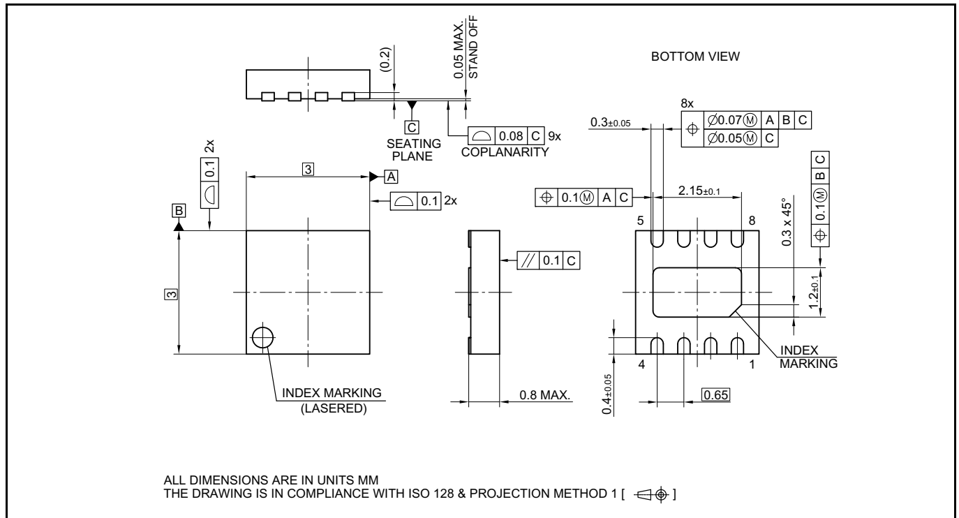
Figure 25 PG-WSN-8-3 outline
