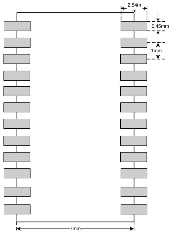
Figure 5. SSOP-24(236mil) Land Pattern Recommendation
