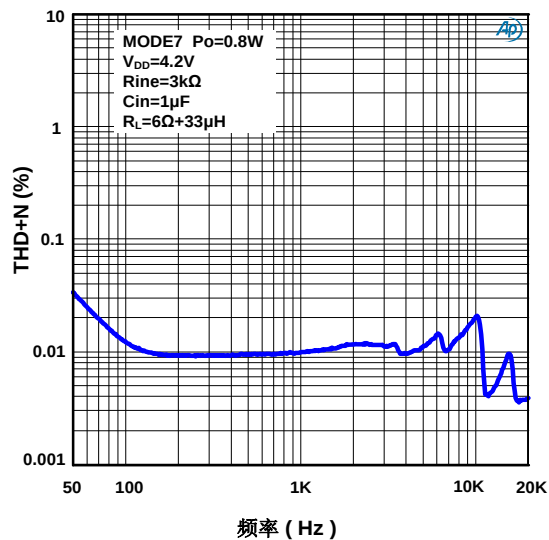
THD+N vs 频率
