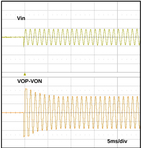
MULTI-LEVEL-AGC 功能启动时序
