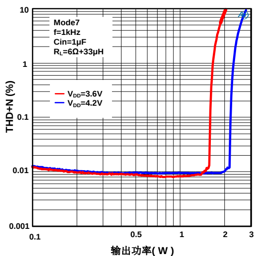
THD+N vs 输出功率
