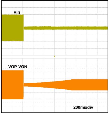
SINGLE-LEVEL-AGC 功能释放时序
