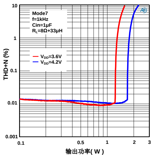
THD+N vs 输出功率
