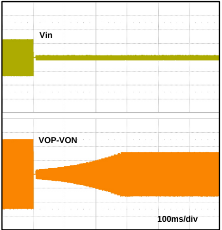
MULTI-LEVEL-AGC 功能释放时序
